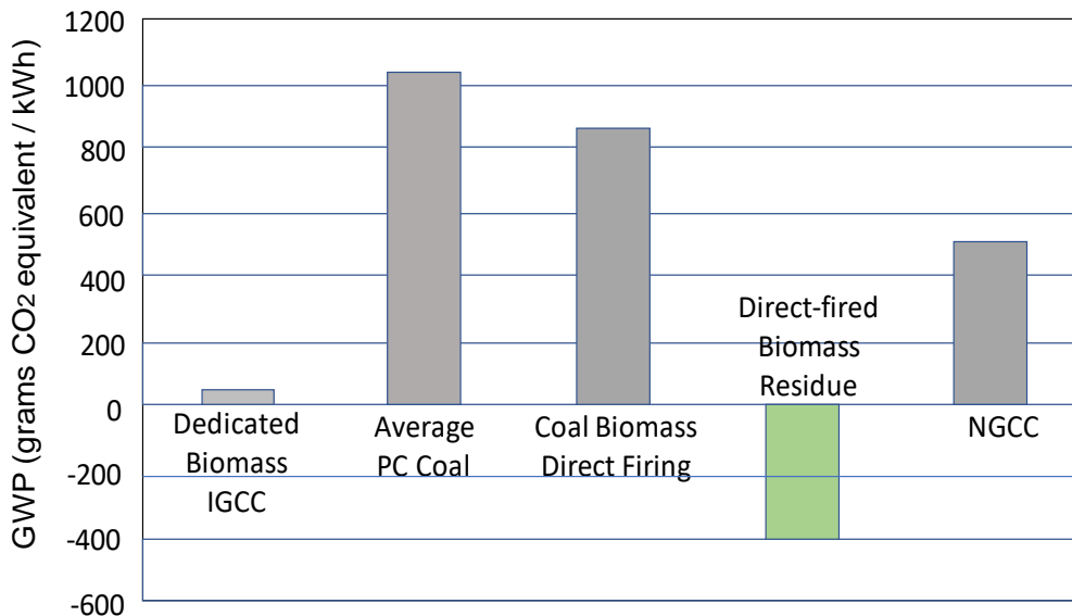
Figure 2. Life cycle assessment [3] shows that thermal conversion of biomass residue to energy results in a net reduction of greenhouse gas equivalent emissions because of the resulting diversion from landfill, where anaerobic decomposition would otherwise produce methane
